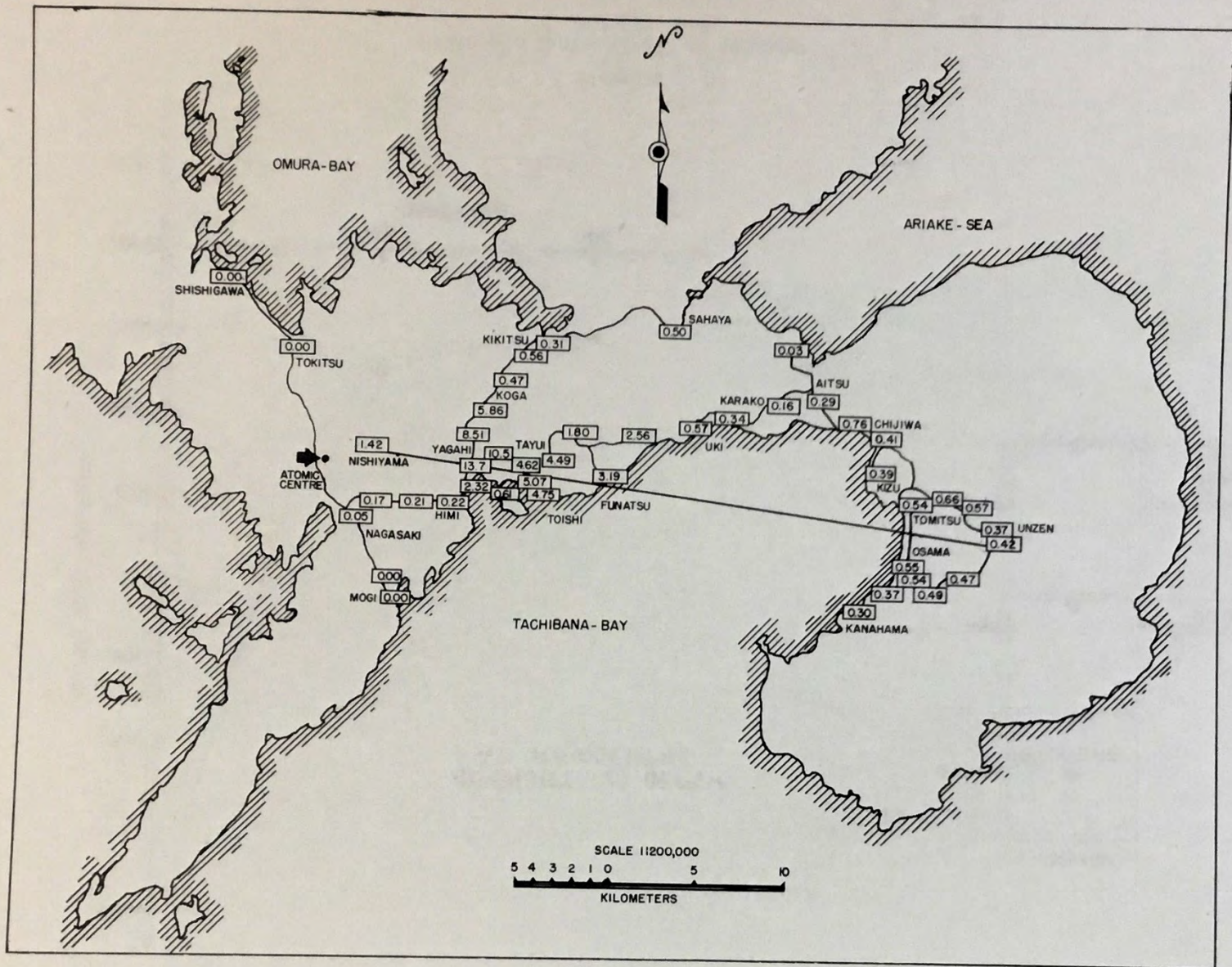
Figure 5 RESIDUAL RADIO-ACTIVITY IN NAGASAKI AND ENVIRONS ( \mu r/hr ) 25 DECEMBER 1945 - 9 JANUARY 1946
