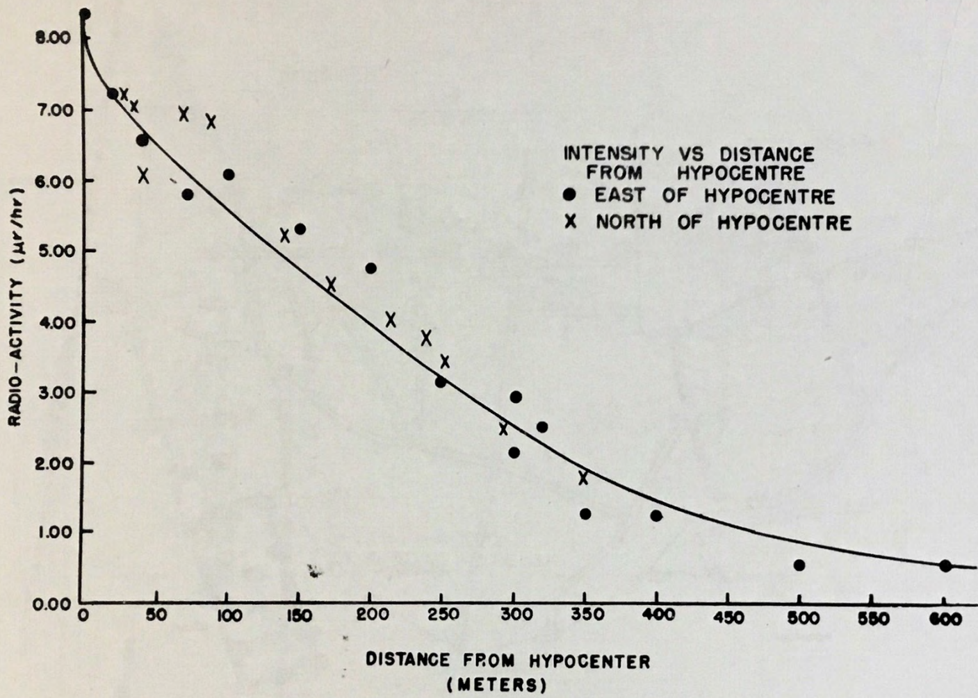
Figure 3 RESIDUAL RADIO-ACTIVITY AT NAGASAKI 26-29 DECEMBER 1945
