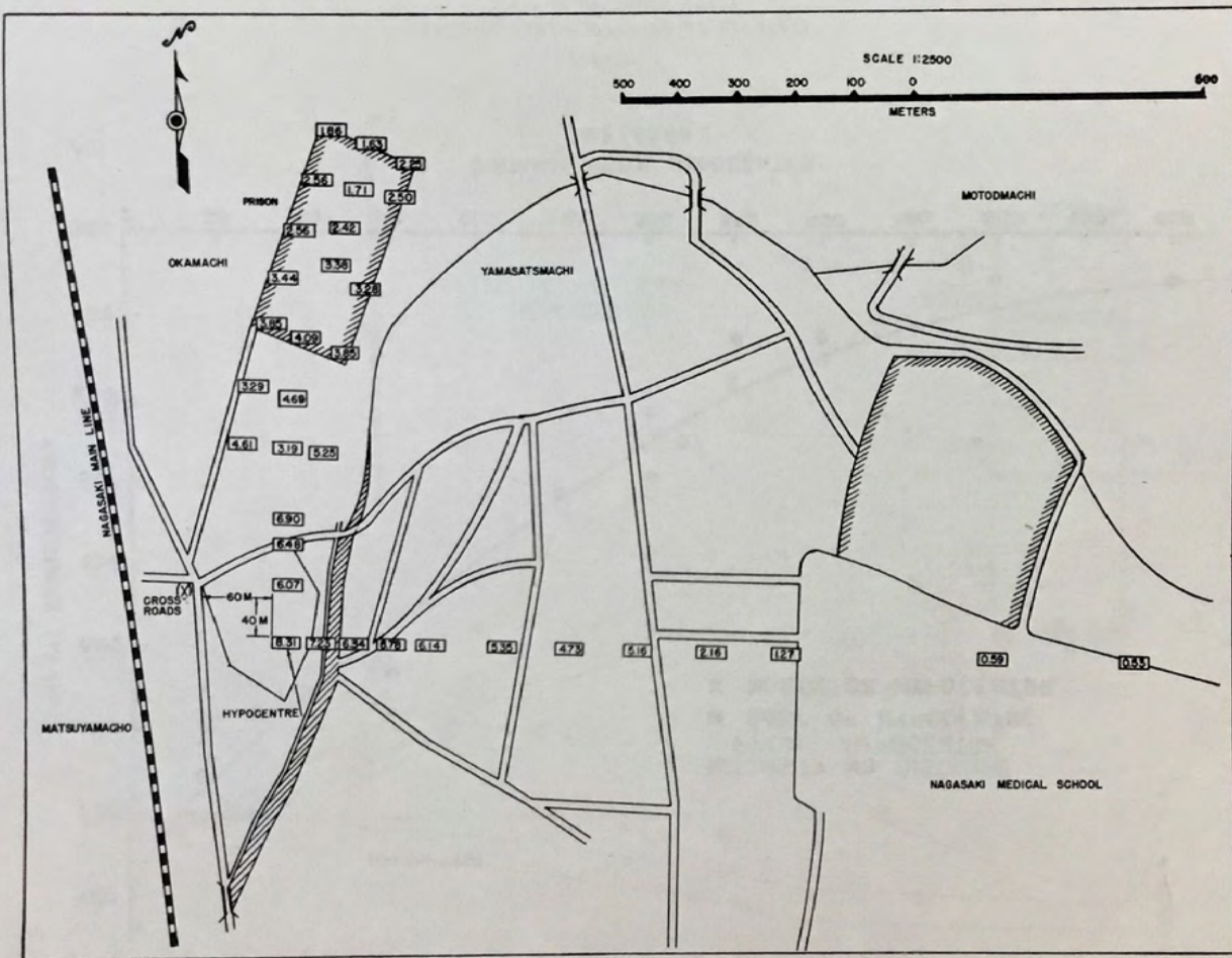
Figure 2 RESIDUAL RADIO-ACTIVITY AT NAGASAKI ( \mu r/hr ) 26-29 DECEMBER 1945
