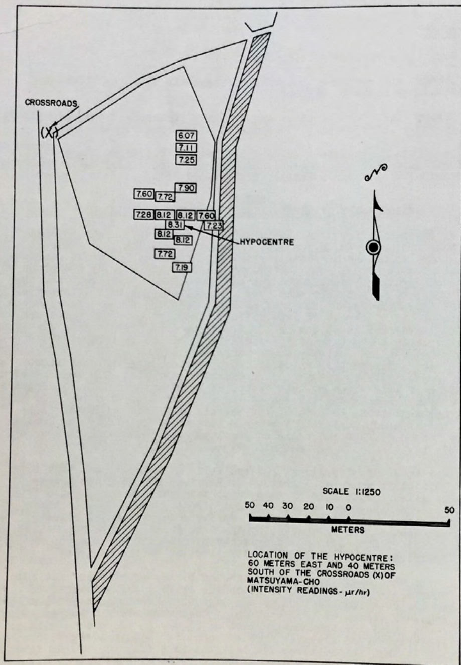
Figure 1 DETERMINATION OF HYPOCENTRE FROM INTENSITY DISTRIBUTION NAGASAKI 27 DECEMBER 1945
