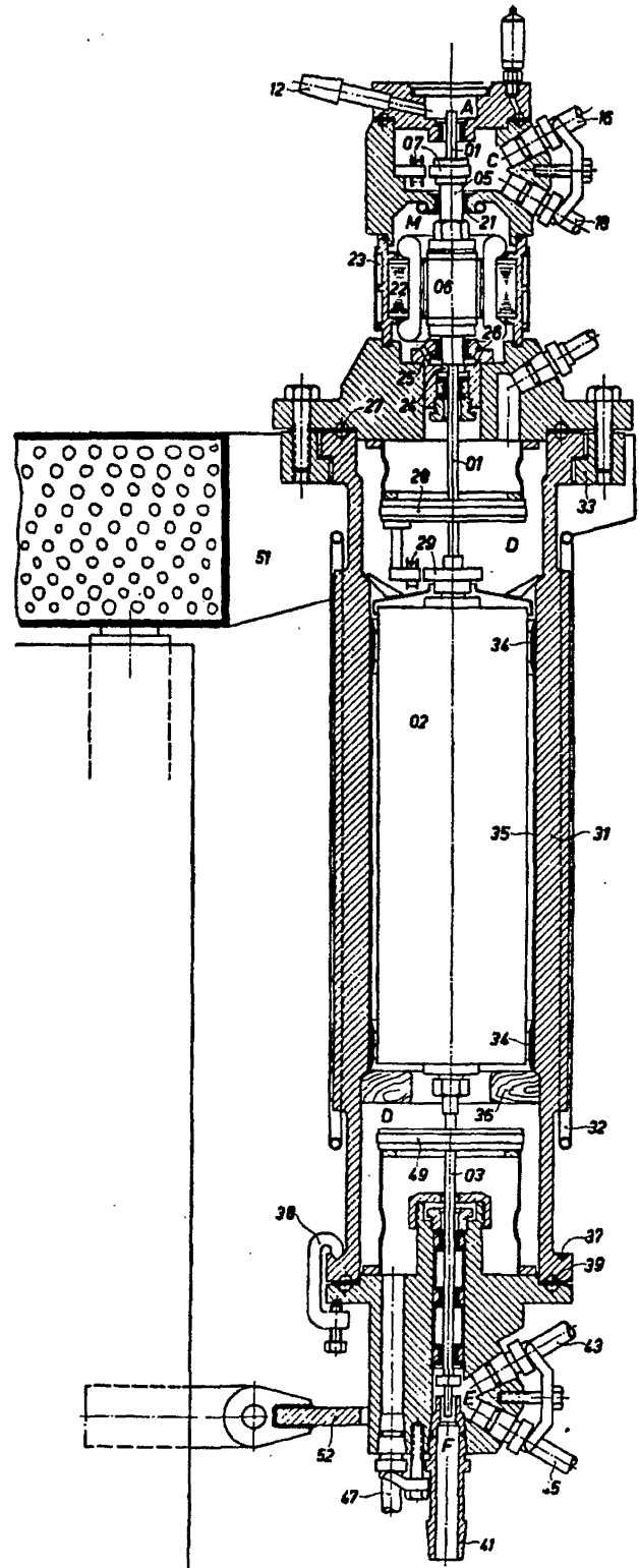
Figure 1 The Present German 300 Meter-Per-Second Gas Centrifuge
