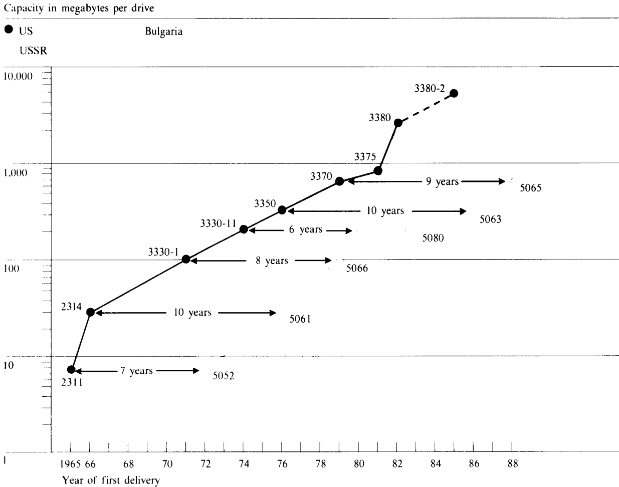
Figure 15 Magnetic Disk Technology: United States Versus USSR, 1965-88
