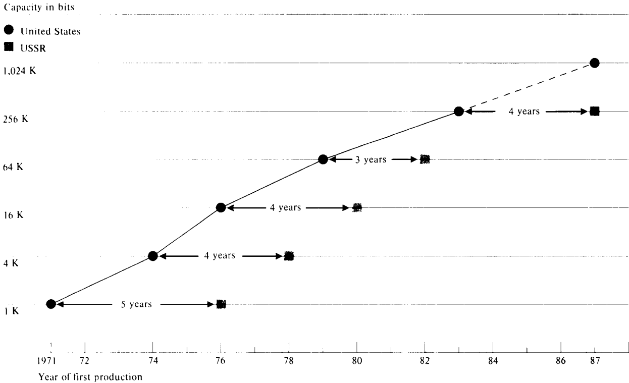
Figure 4 Semiconductor Memory Technology: United States Versus USSR, 1971-87 a
