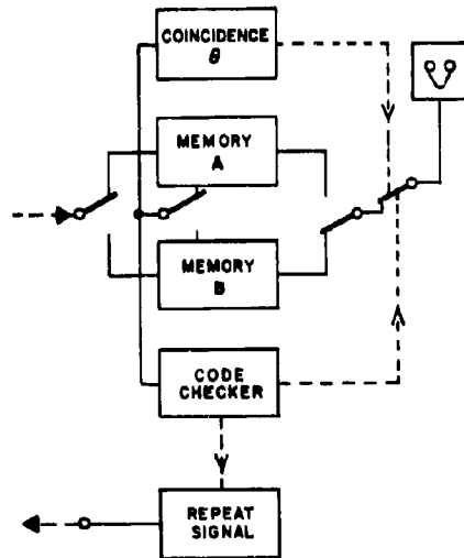
Figure 2.—Receiver Logic.
