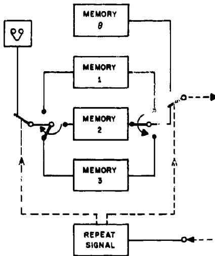
Figure 1.—Transmission Logic.
