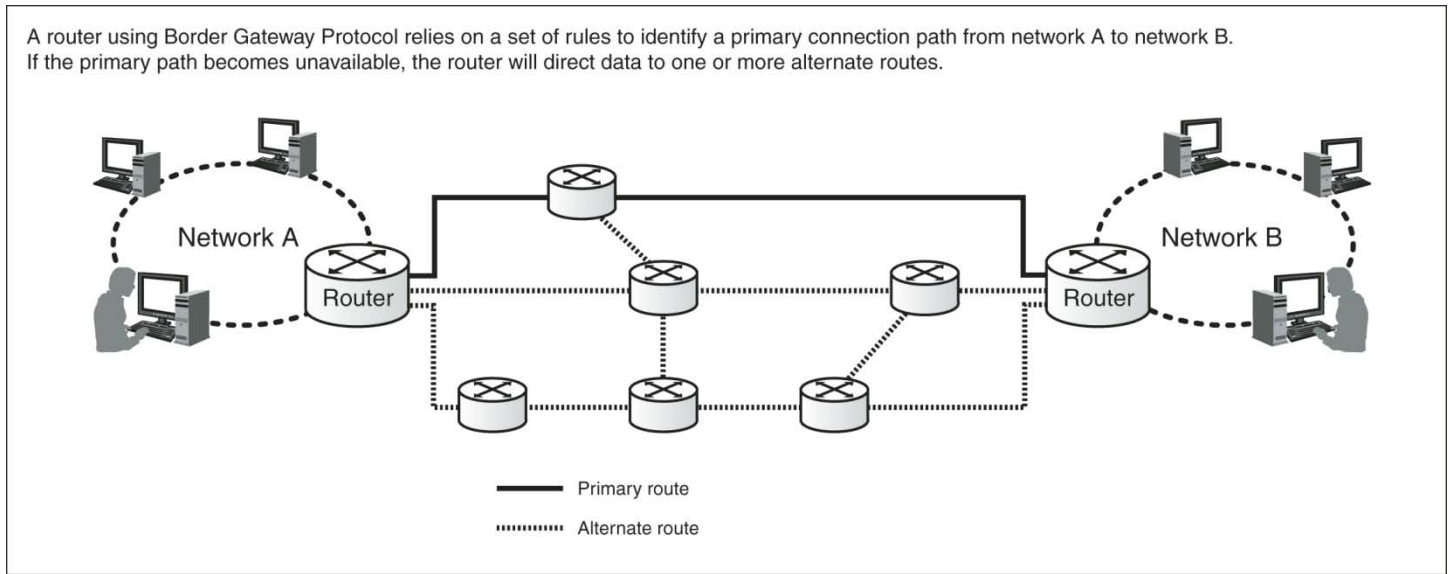
Figure 4: Example of Dynamic Routing Using Border Gateway Protocol
