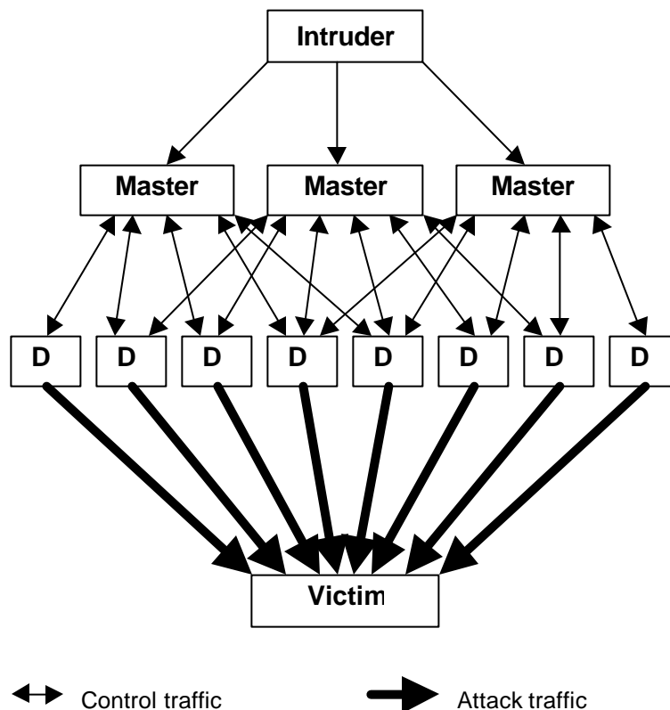
Figure 1 – Distributed-Systems Attack
