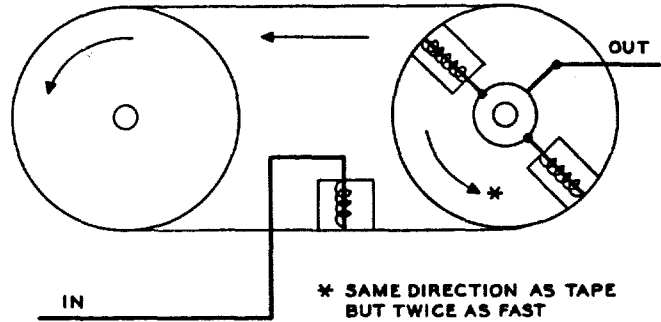
Figure 16 - Time Inversion
