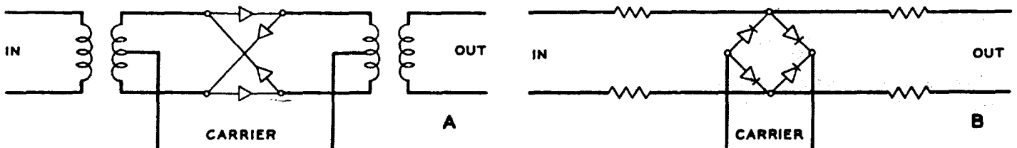
Figure 6 - Modulators
