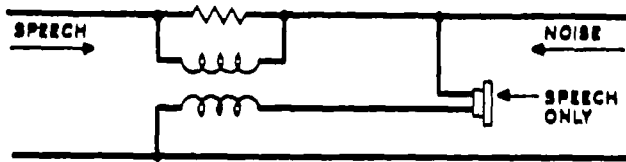
Figure 34 - Directional Discrimination
