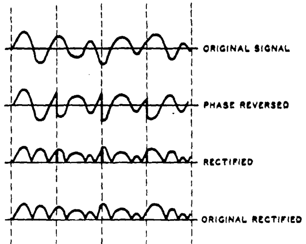
Figure 32 - Illustrating Action of Rectifier
