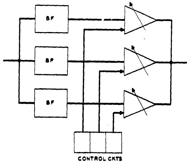
Figure 19 - Subband Level Modulation
