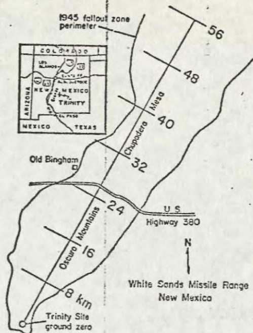
Fig. 1. Sampling transect utilized for the radioecological resurvey of Trinity.
