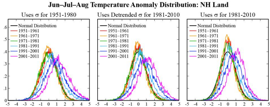
Figure 19. Distributions of Northern Hemisphere Summer Temperature Anomalies over Land by Decade (Source: Hansen et al, 2012a).
