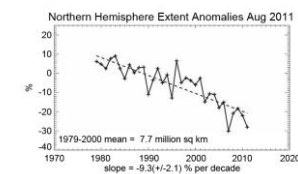
Decreasing Arctic Sea Ice Extent (NSIDC)
