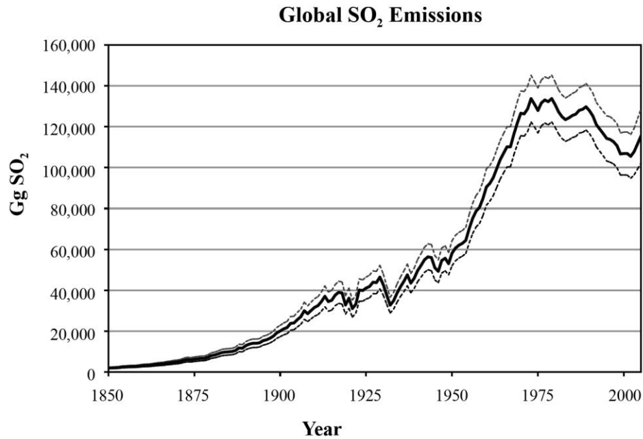
Figure 11. Global Sulfur Dioxide Emissions from Fuel Combustion and Process Emissions with Central Value (solid line) and Upper and Lower Uncertainty Bounds (dotted lines).
