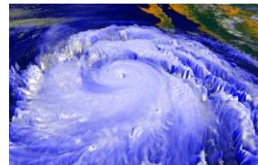
Potential for Increased Storm Intensity
