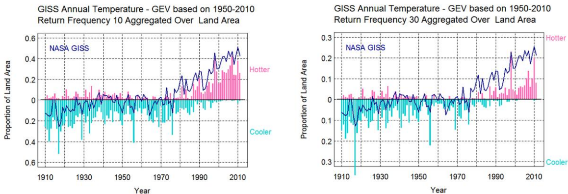
Figure 20. Comparison of Global Mean Land Surface Temperature Prevalence of 10- (left) and 30-year (right) Extremes.
