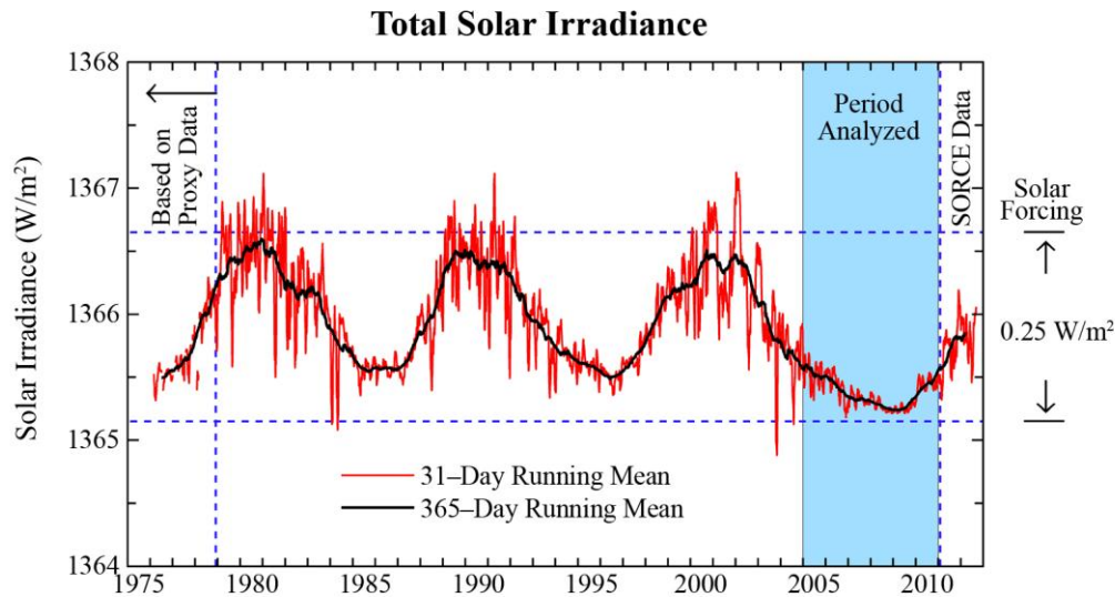
Figure 1. Solar Irradiance.
