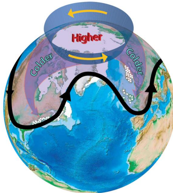
Figure 36. Negative Arctic Oscillation.
