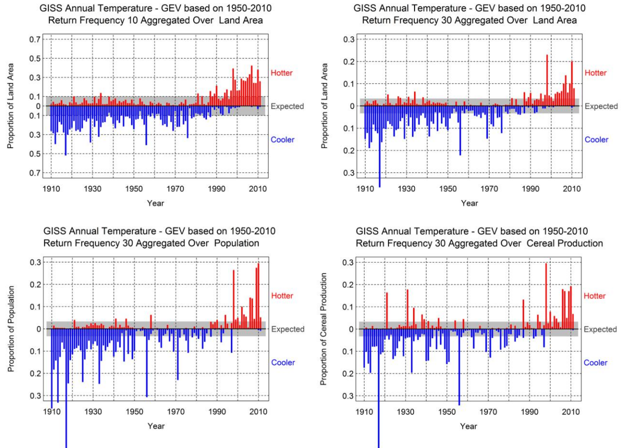
Figure 18. Trends in the Prevalence of Extreme Annual Average Temperature Using 1950-2010 Baseline.
