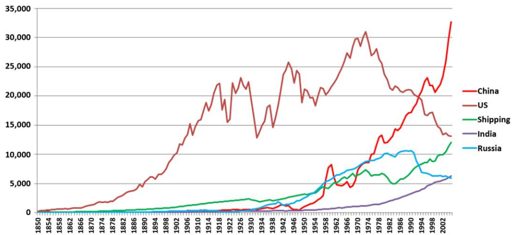
Figure 12. Top 5 SO 2 Emitters (Gg SO 2 ).
